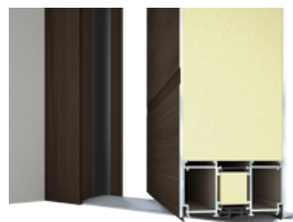
Cutaway Detail
