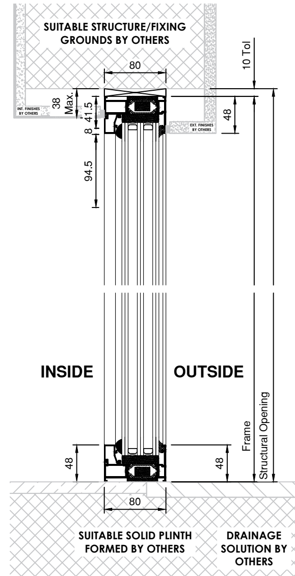
SECTION C-C
