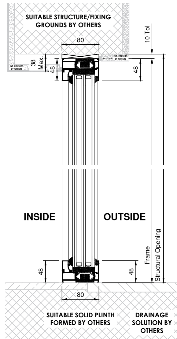
SECTION C-C
